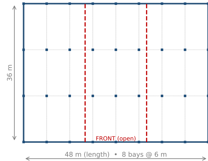
FLOOR PLAN
