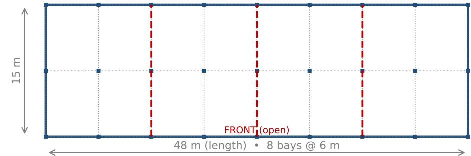
FLOOR PLAN
