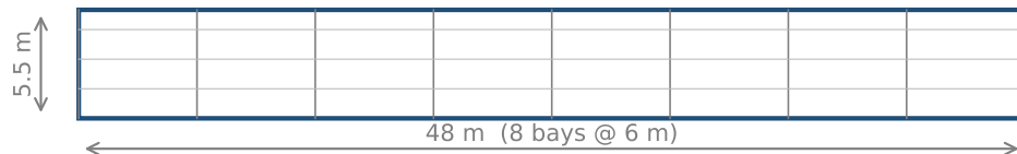
SIDE ELEVATION
